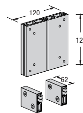
E 185 Monitor-Adapter
